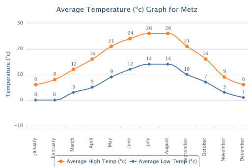
Figure 1. Average minimum (blue) and maximum (orange) temperatures in Metz, France.
